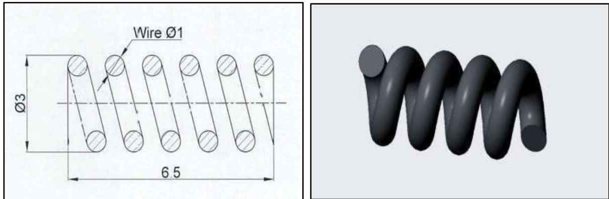
Figure 6.12: SPRING (ANTI-STATIC)
