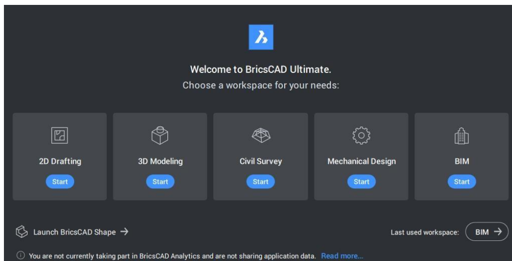
Figure 4.1: BricsCAD Launcher
