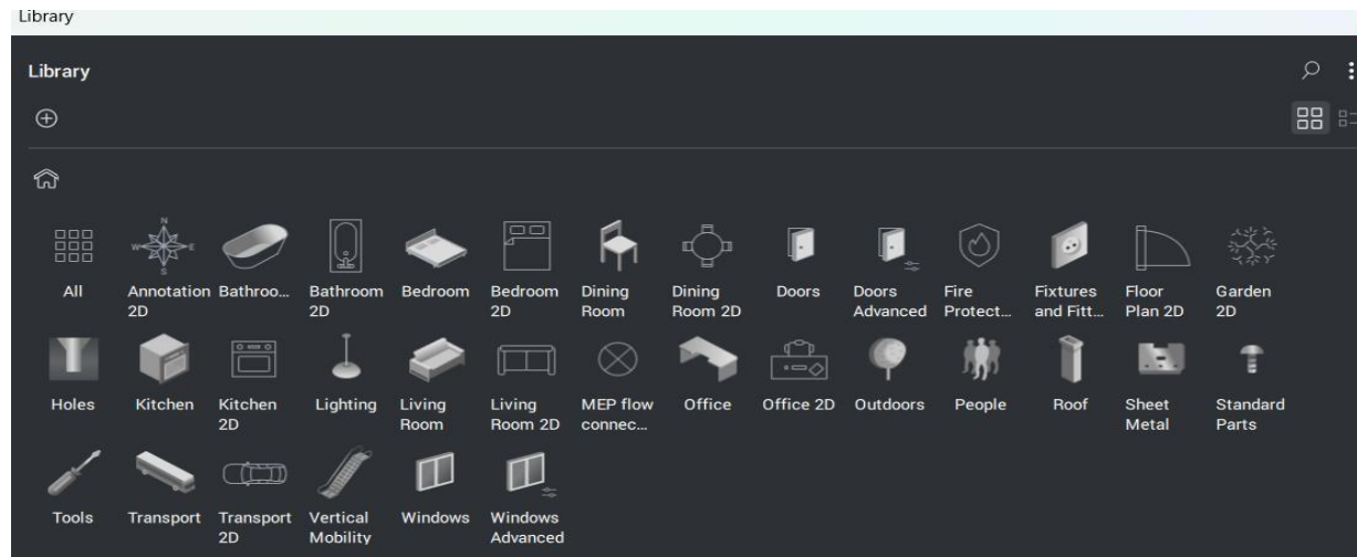
Figure 4.5: Library
