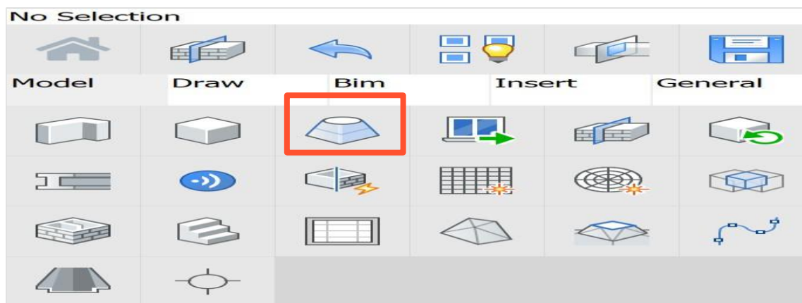
fig 4.6: Quad Cursor
