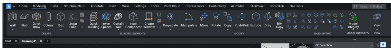
Figure 4.2: Ribbon Menu
