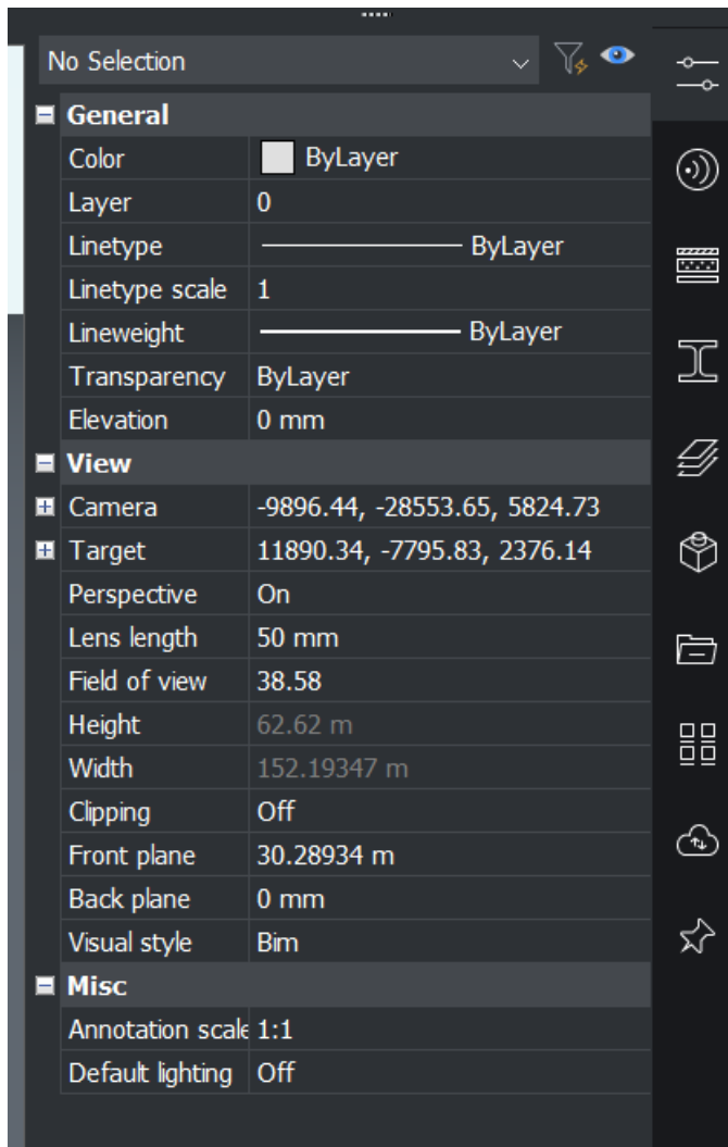
Figure 4.4: Property Panel
